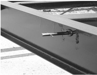
Fig. 1-Through Frame Crank Extension w/pin.
